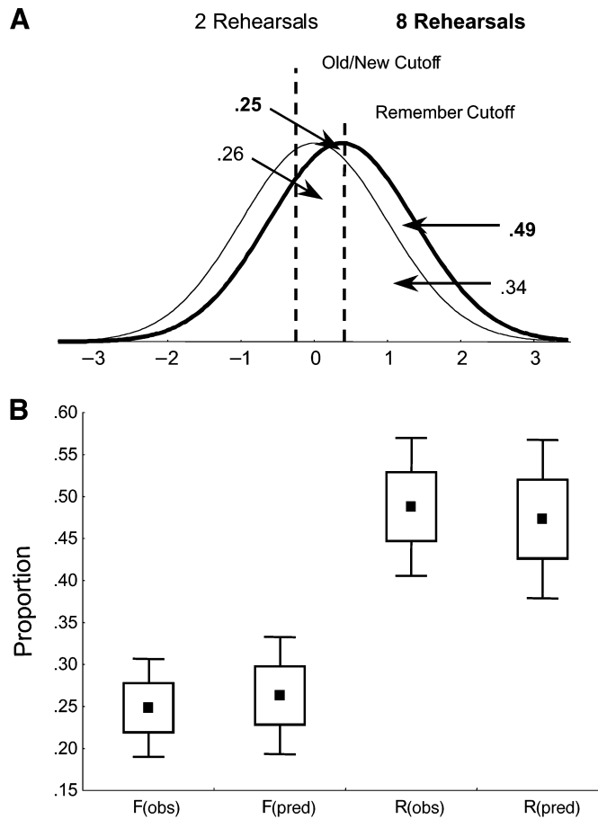
Figure 4. Predictions of the two-criterion signal detection model for incorrect Brown–Peterson data. Panel A illustrates the predicted proportion of familiar and remember responses for the eight-rehearsal condition assuming equivalent standard deviations of the two- and eight-rehearsal item distributions. Heavy curve is for eight rehearsals; light, for two. Panel B shows the mean difference between predicted (pred) and observed (obs) data for individual subjects. F is familiarity, and R is remember rate.
